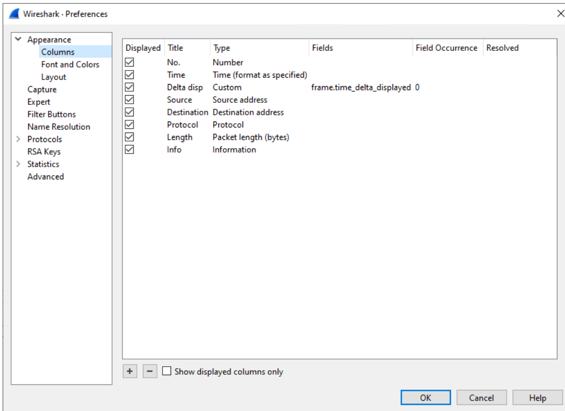
Figure 124. Column preferences
