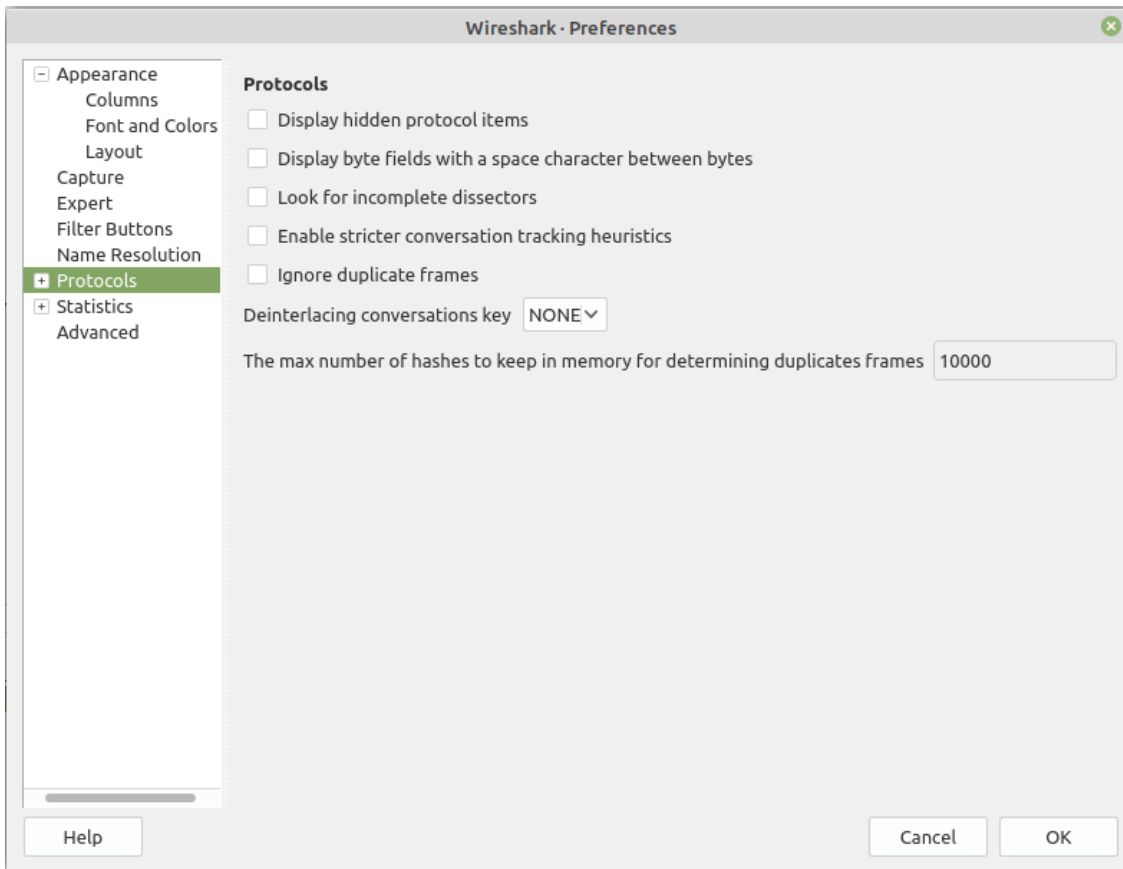
Figure 131. Protocol preferences
