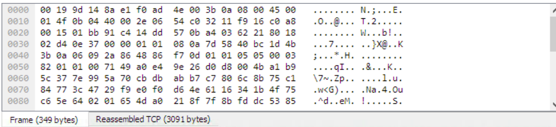
Figure 77. The “Packet Bytes” pane with a reassembled tab
