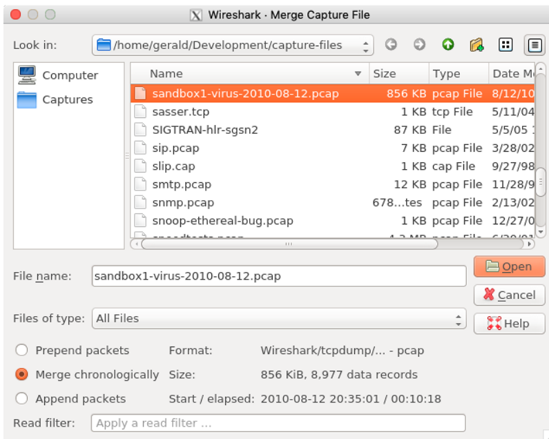
Figure 41. “Merge” on Linux and UNIX
